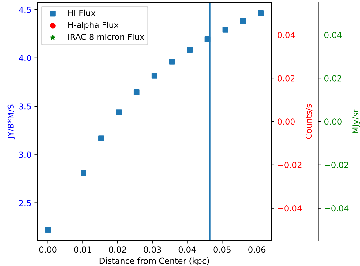
Flux of HI vs. H-alpha in Galaxy: IC10 - Region 20
