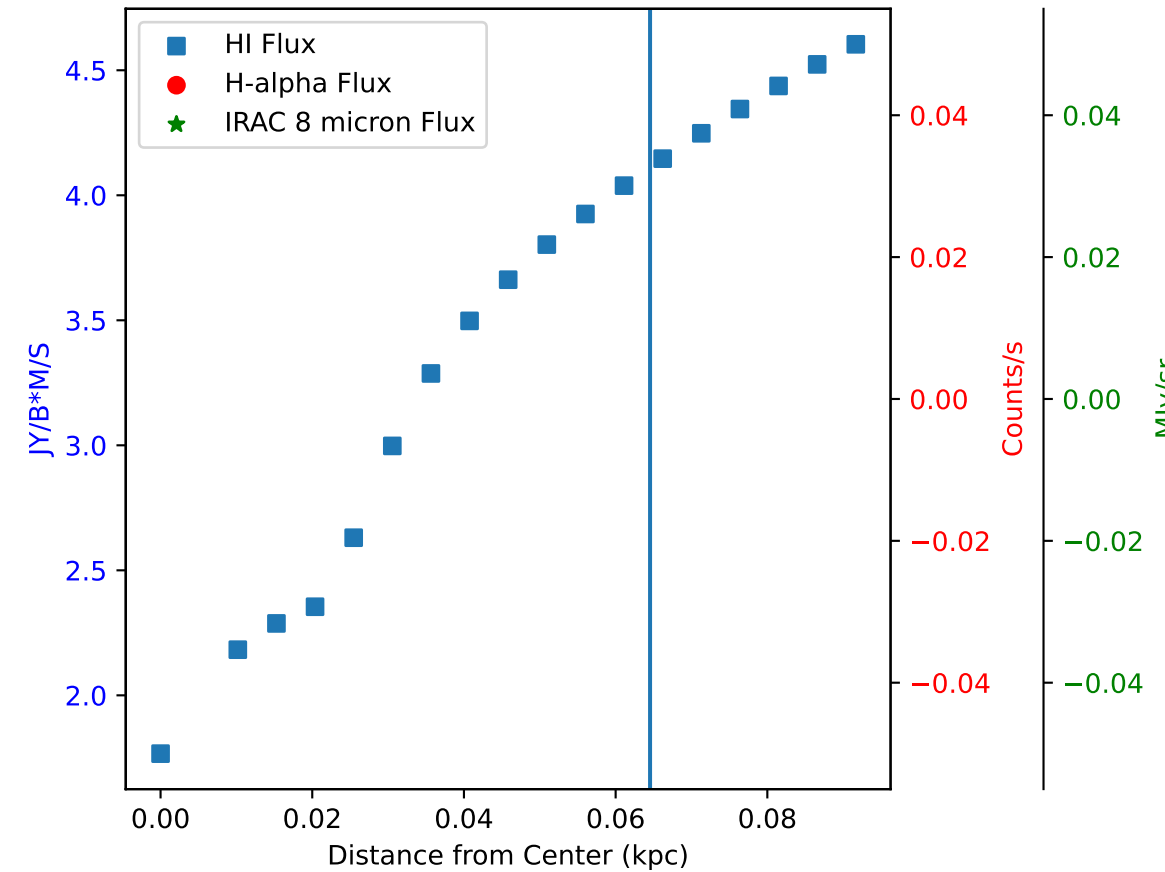
Flux of HI vs. H-alpha in Galaxy: IC10 - Region 4
