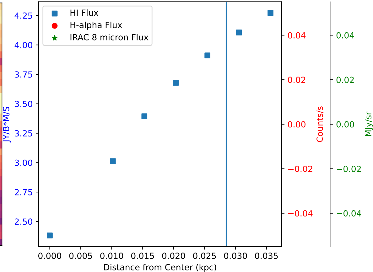
Flux of HI vs. H-alpha in Galaxy: IC10 - Region 18
