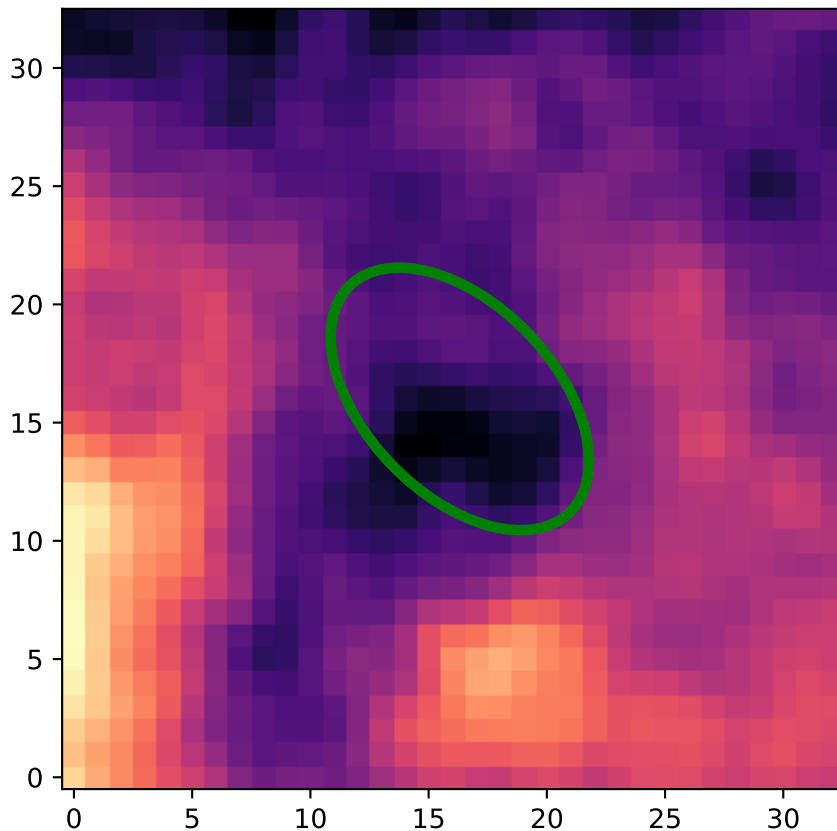
Region: 11 HI - Type 1
