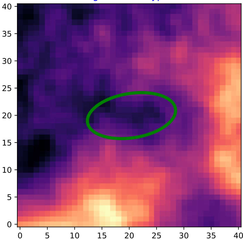
Region: 2 HI - Type 2
