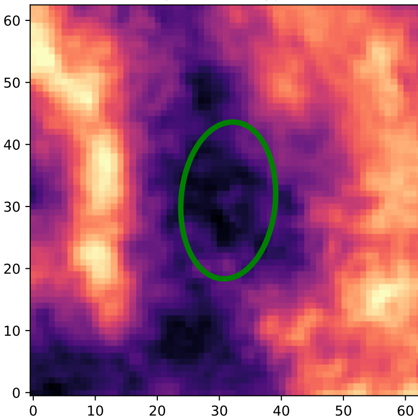
Region: 4 HI - Type 1
