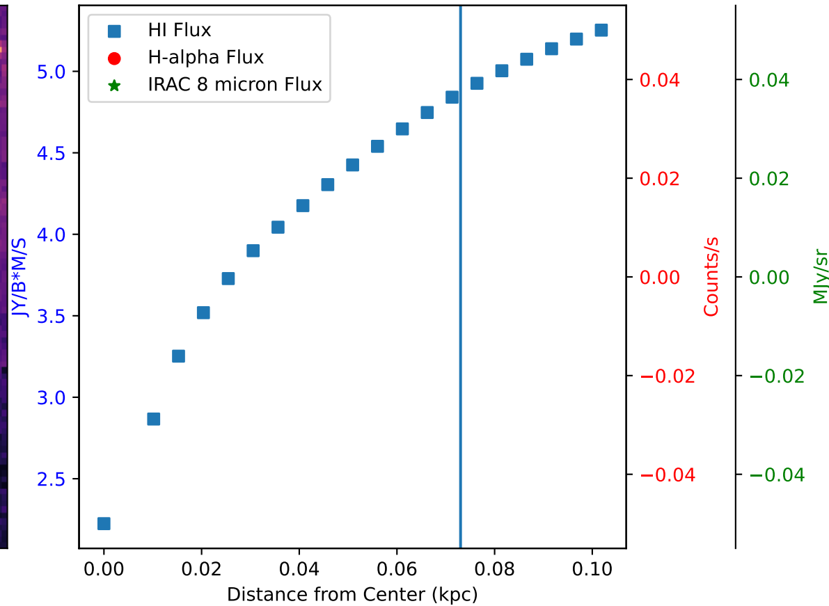
Flux of HI vs. H-alpha in Galaxy: IC10 - Region 14
