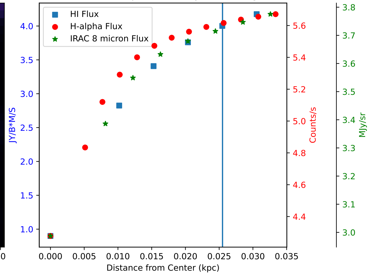
Flux of HI vs. H-alpha in Galaxy: IC10 - Region 9
