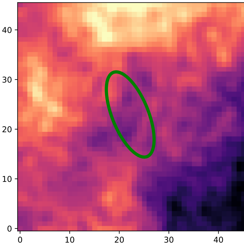
Region: 20 HI - Type 2
