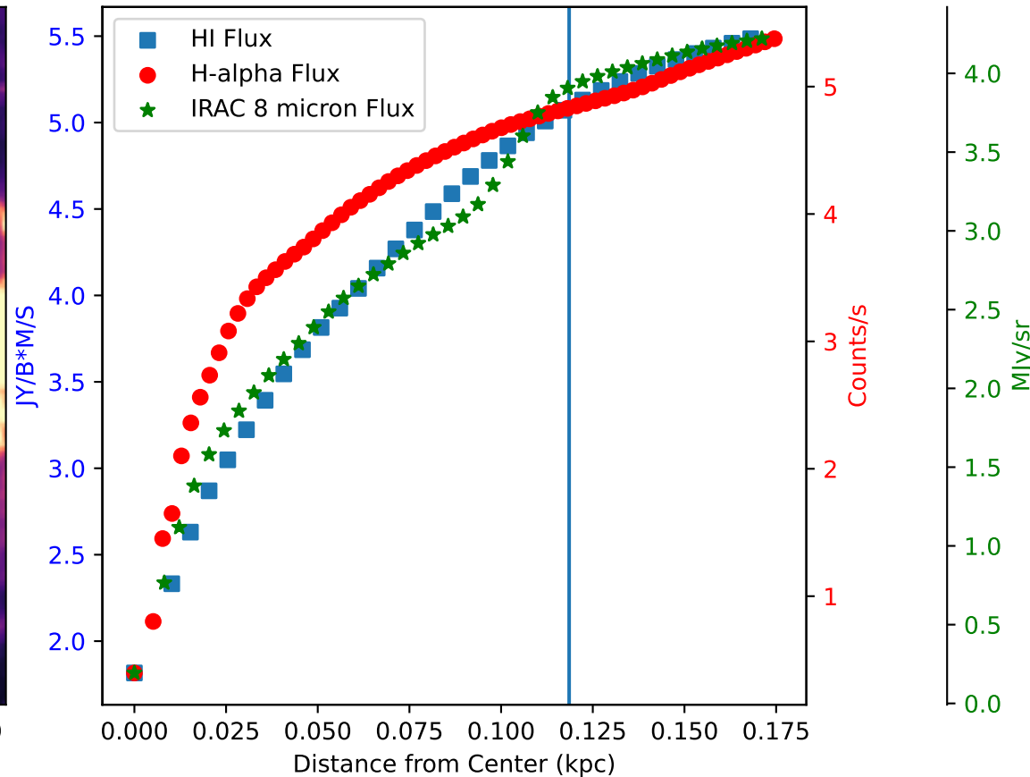
Flux of HI vs. H-alpha in Galaxy: IC10 - Region 10
