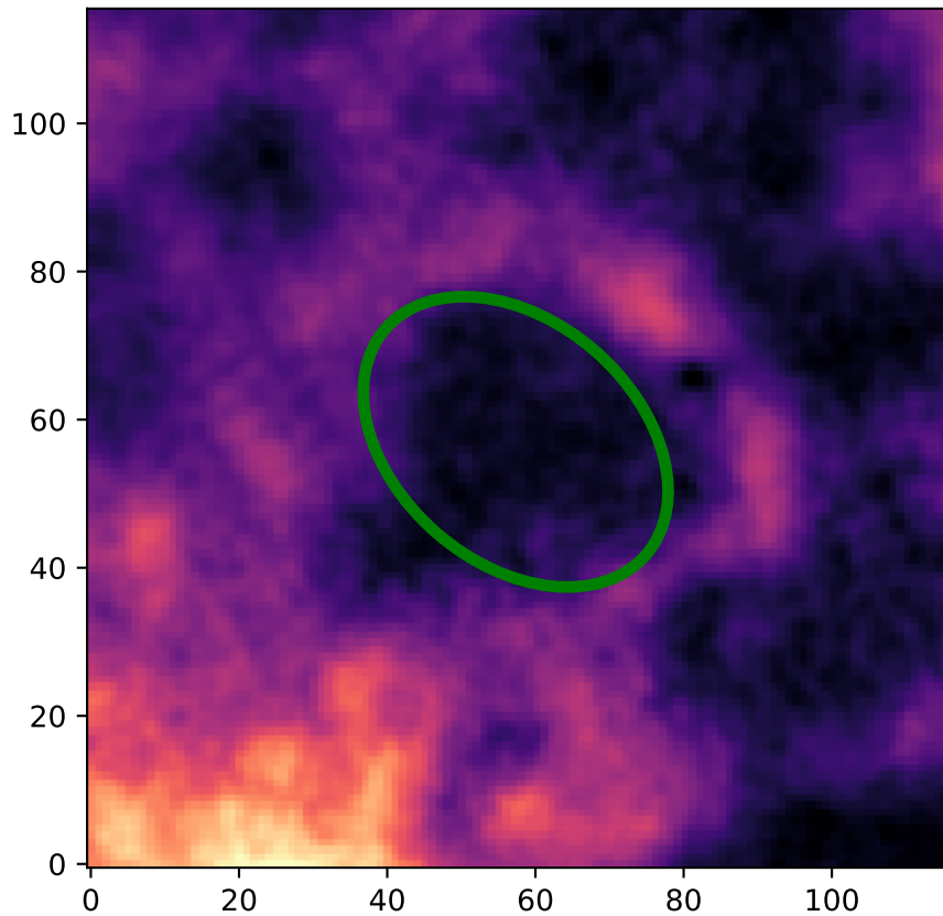
Region: 10 HI - Type 1
