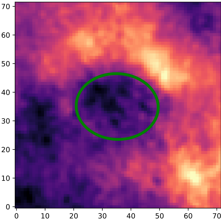
Region: 14 HI - Type 1
