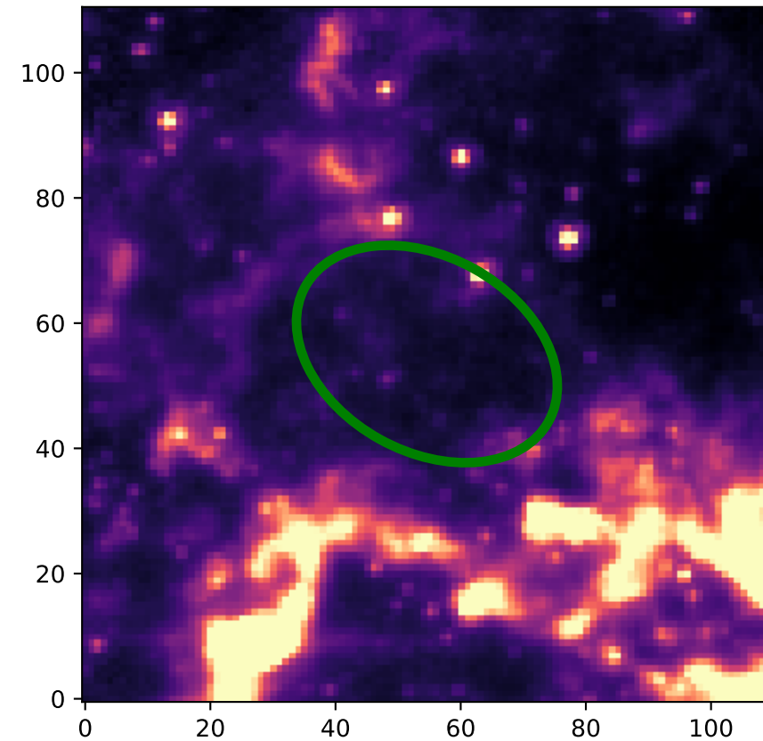
IRAC 8 micron - Classification: Bubble-Like
