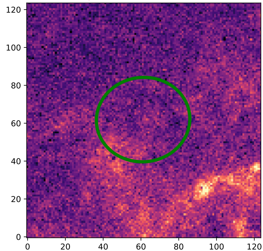
H-alpha - Classification: Diffuse
