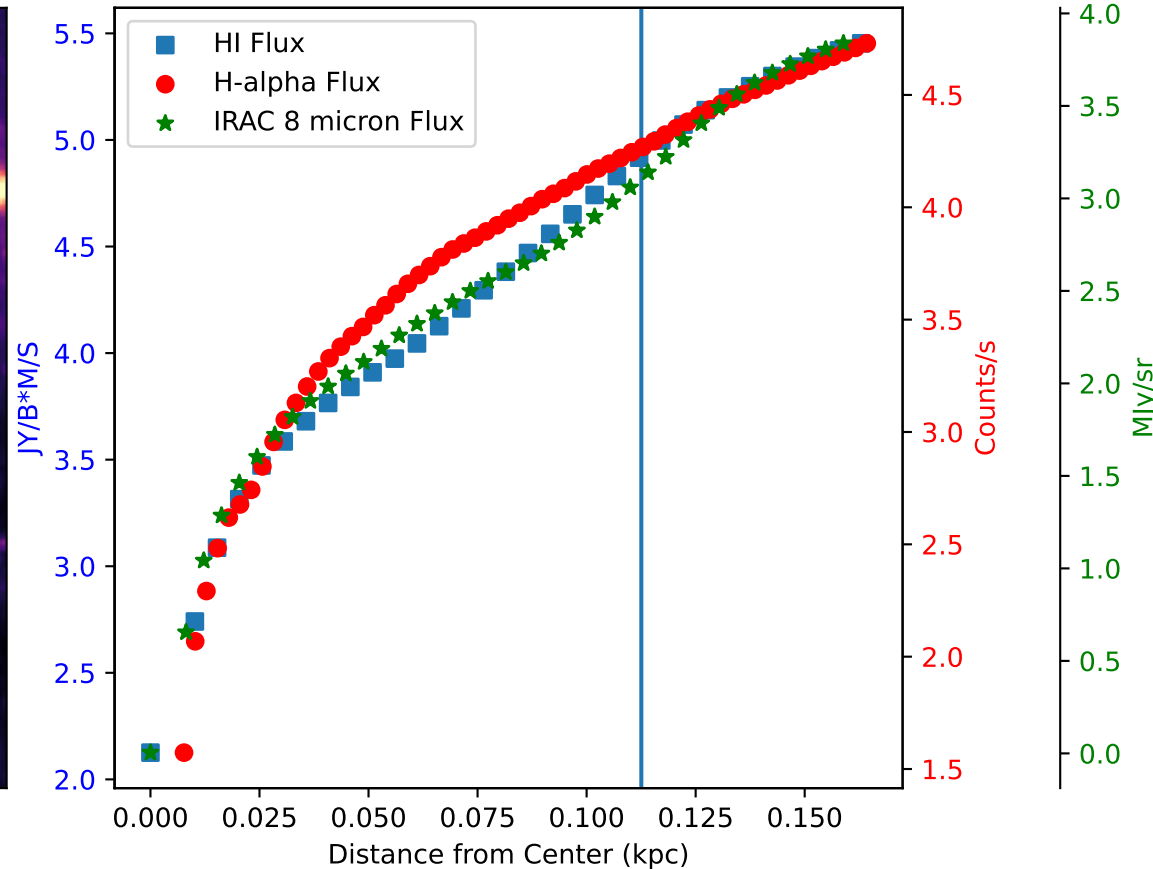
Flux of HI vs. H-alpha in Galaxy: IC10 - Region 8
