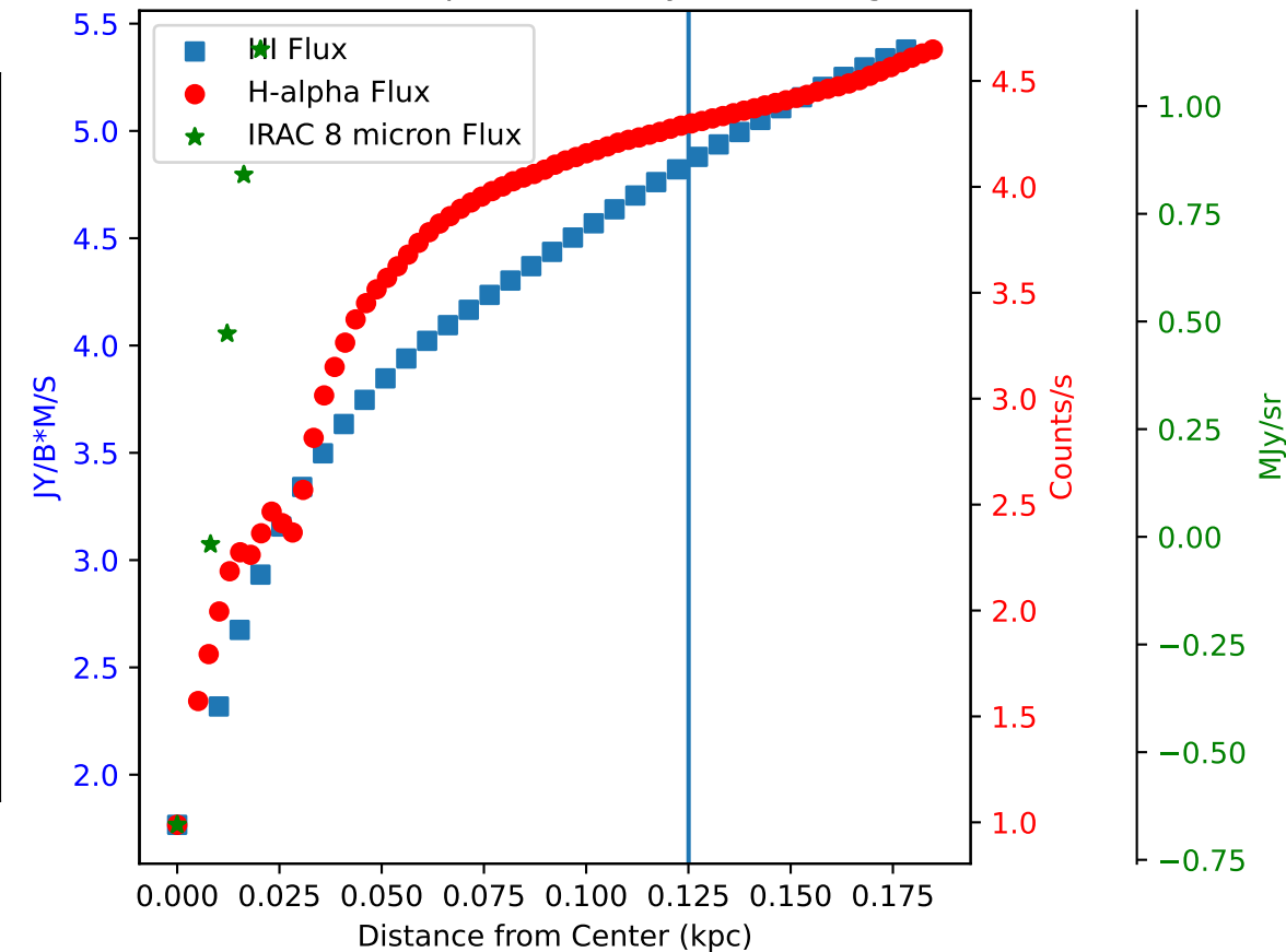
Flux of HI vs. H-alpha in Galaxy: IC10 - Region 3
