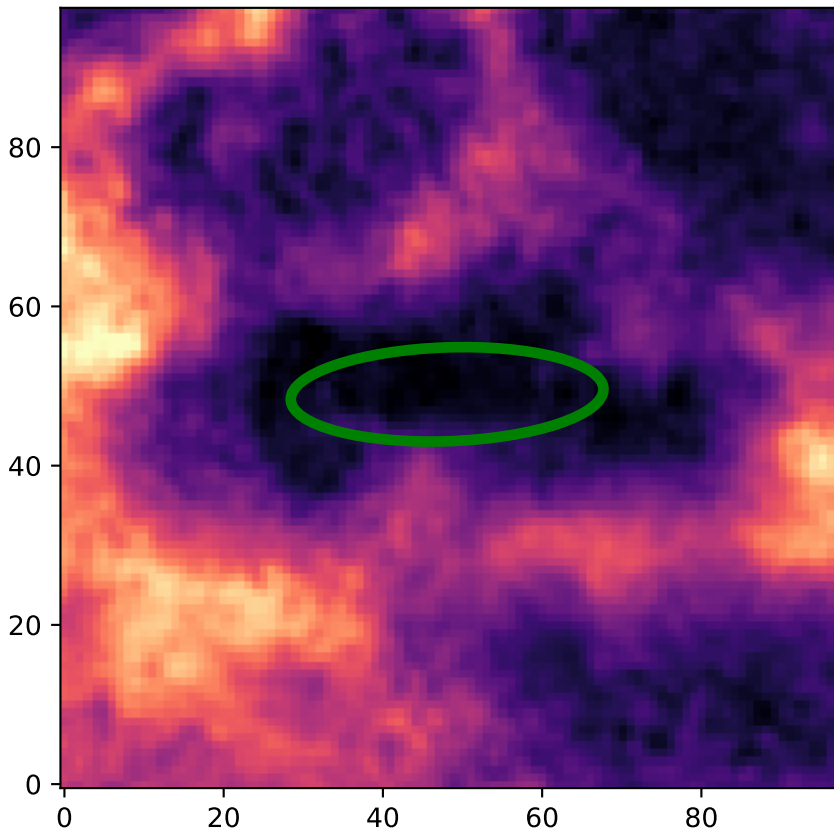
Region: 5 HI - Type 1
