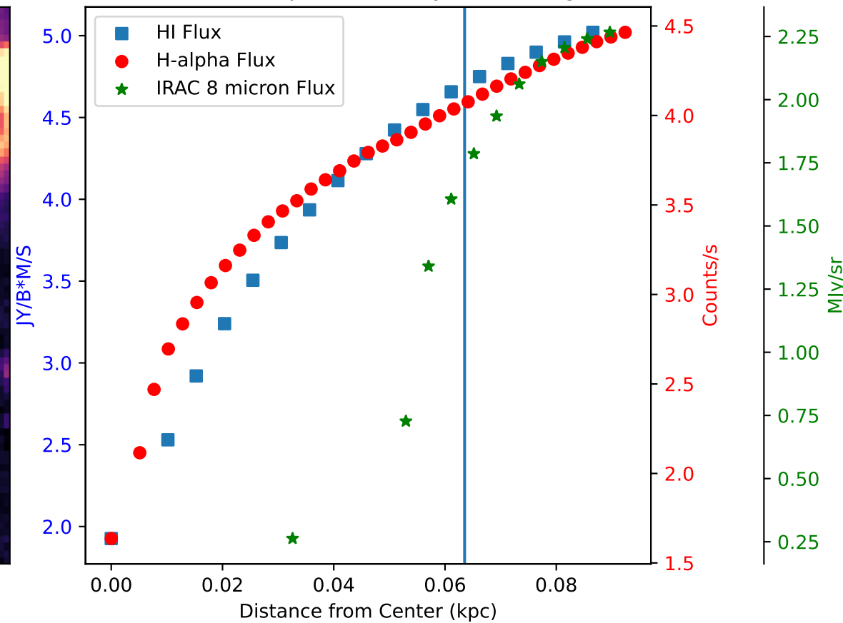
Flux of HI vs. H-alpha in Galaxy: IC10 - Region 15
