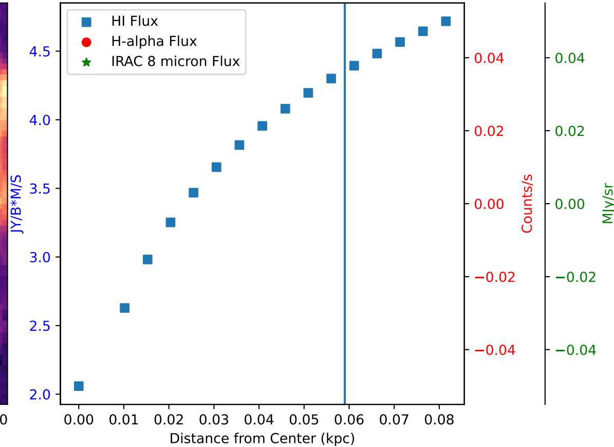
Flux of HI vs. H-alpha in Galaxy: IC10 - Region 16
