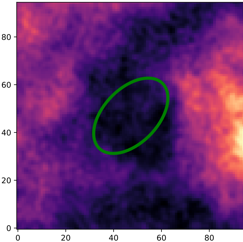
Region: 17 HI - Type 1
