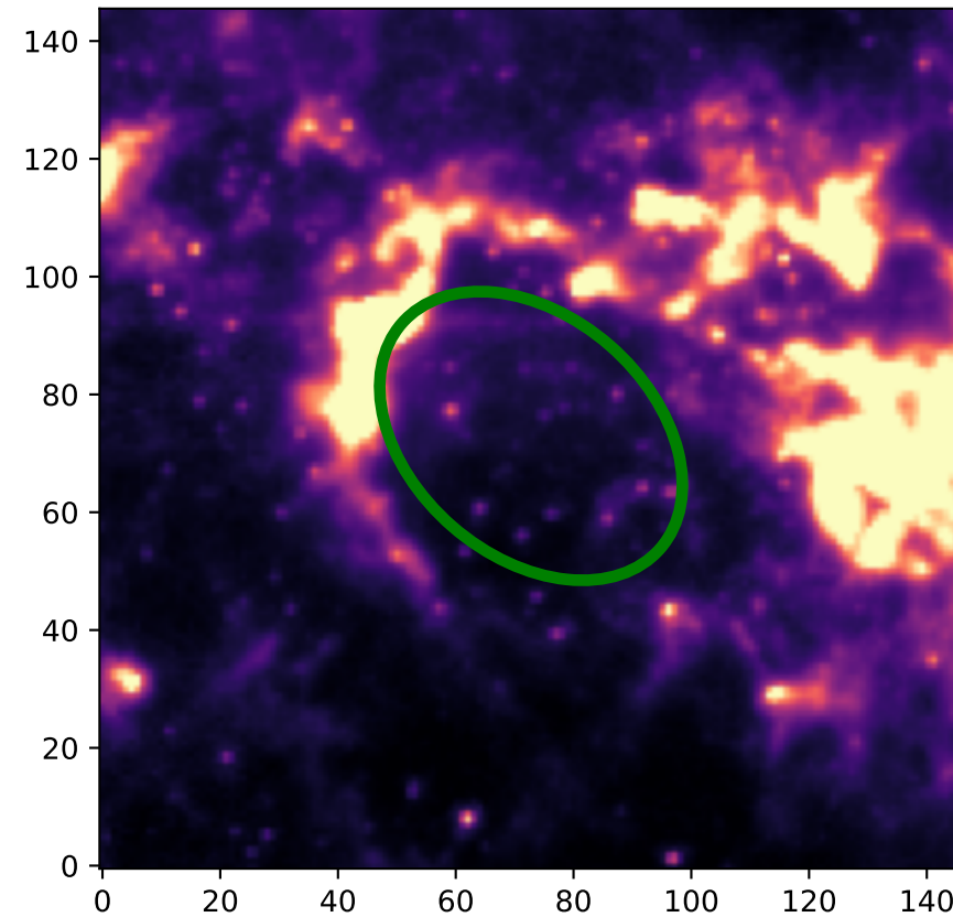
IRAC 8 micron - Classification: Bubble-Like
