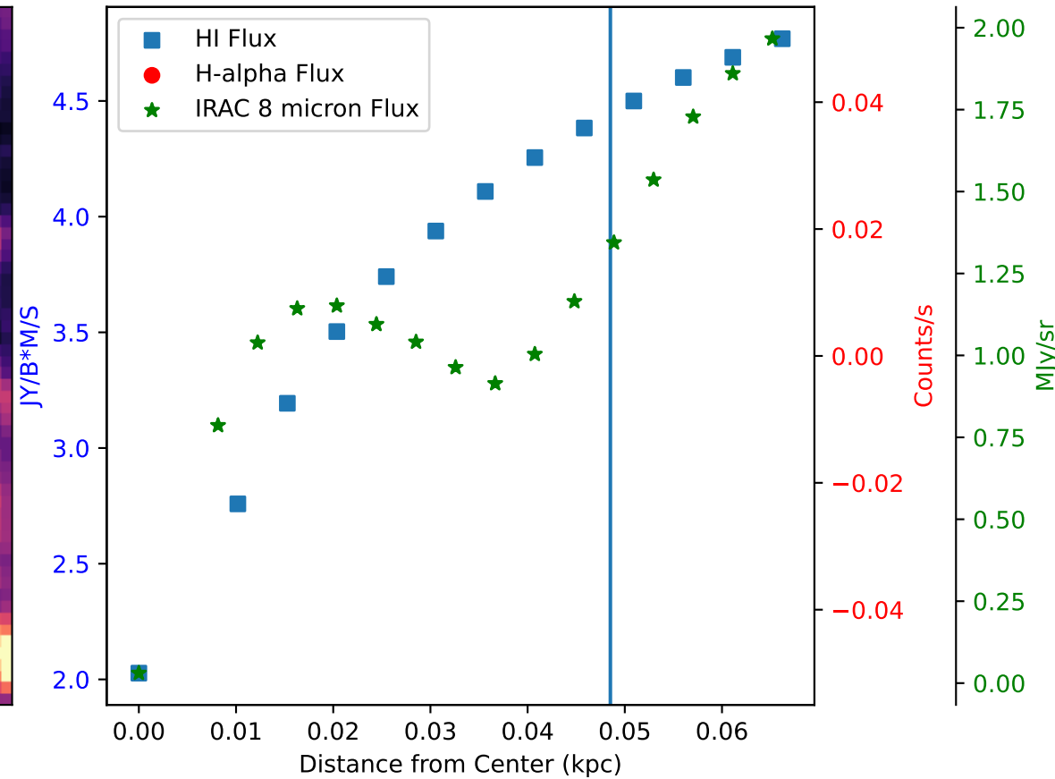
Flux of HI vs. H-alpha in Galaxy: IC10 - Region 13
