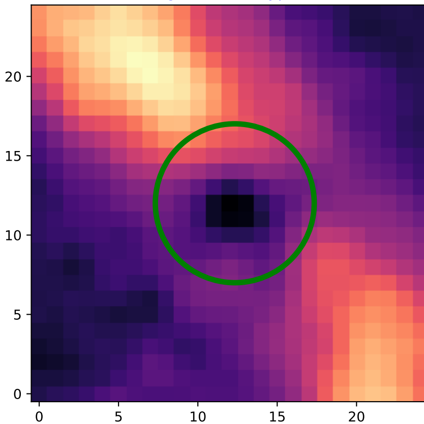
Region: 9 HI - Type 2
