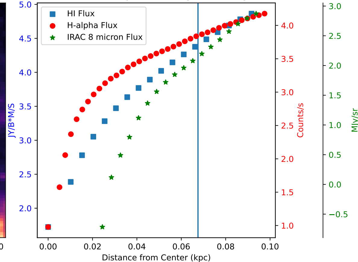
Flux of HI vs. H-alpha in Galaxy: IC10 - Region 7
