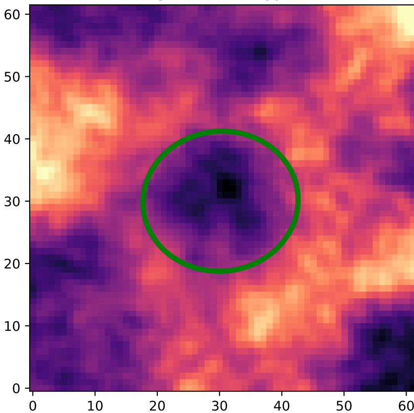
Region: 15 HI - Type 1
