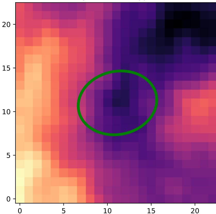
Region: 12 HI - Type 1
