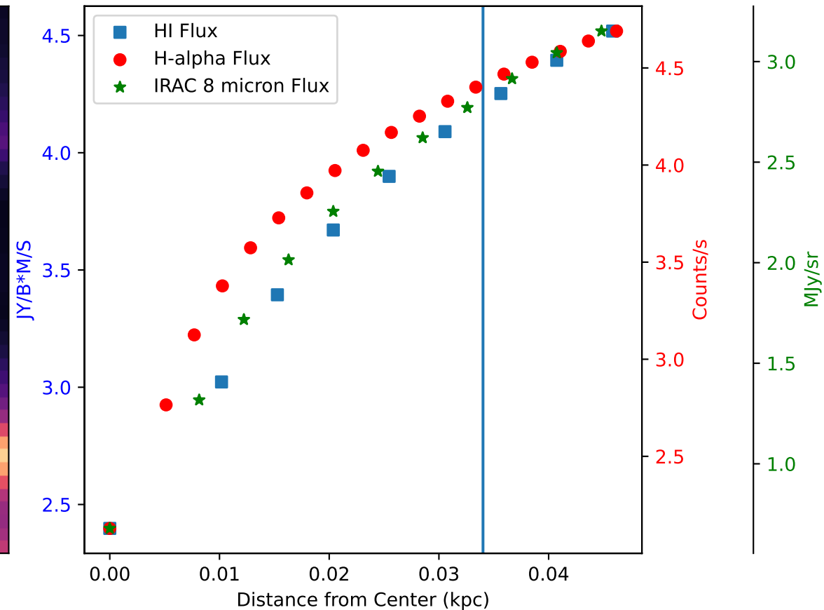
Flux of HI vs. H-alpha in Galaxy: IC10 - Region 11
