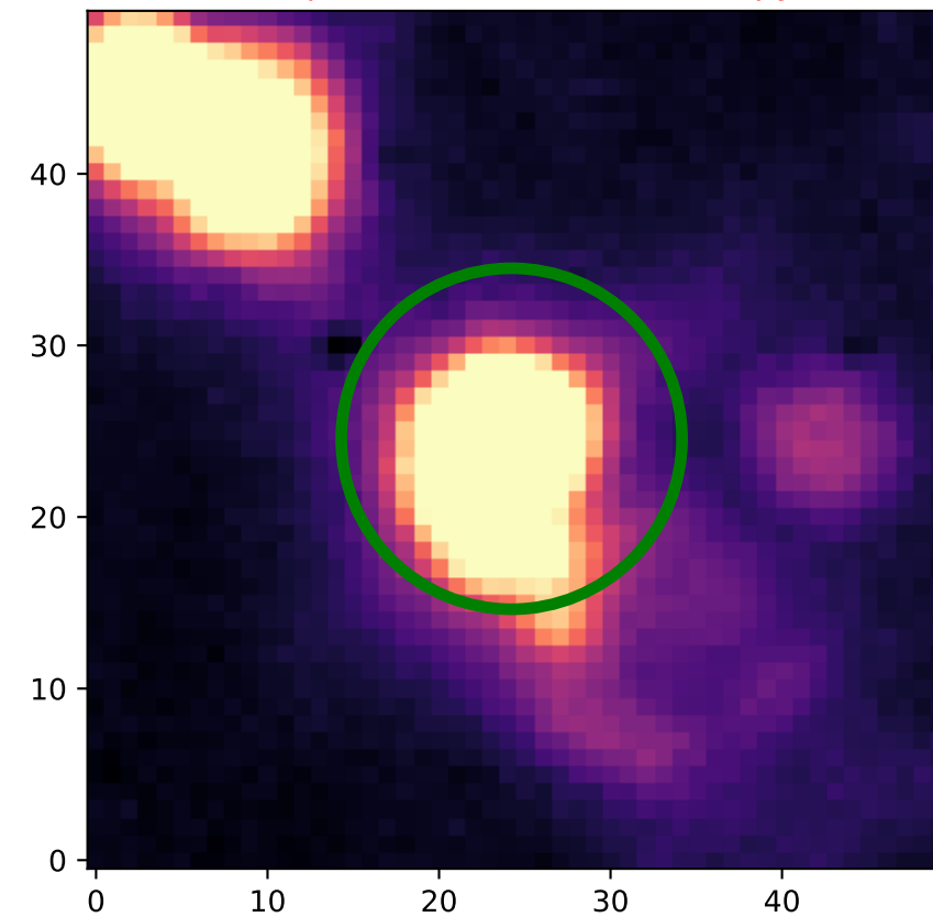
H-alpha - Classification: Clumpy
