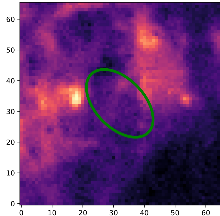
H-alpha - Classification: Bubble-Like
