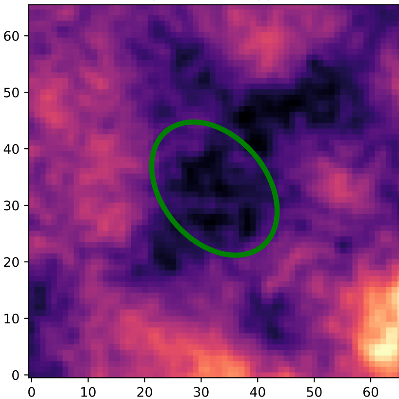
Region: 19 HI - Type 1
