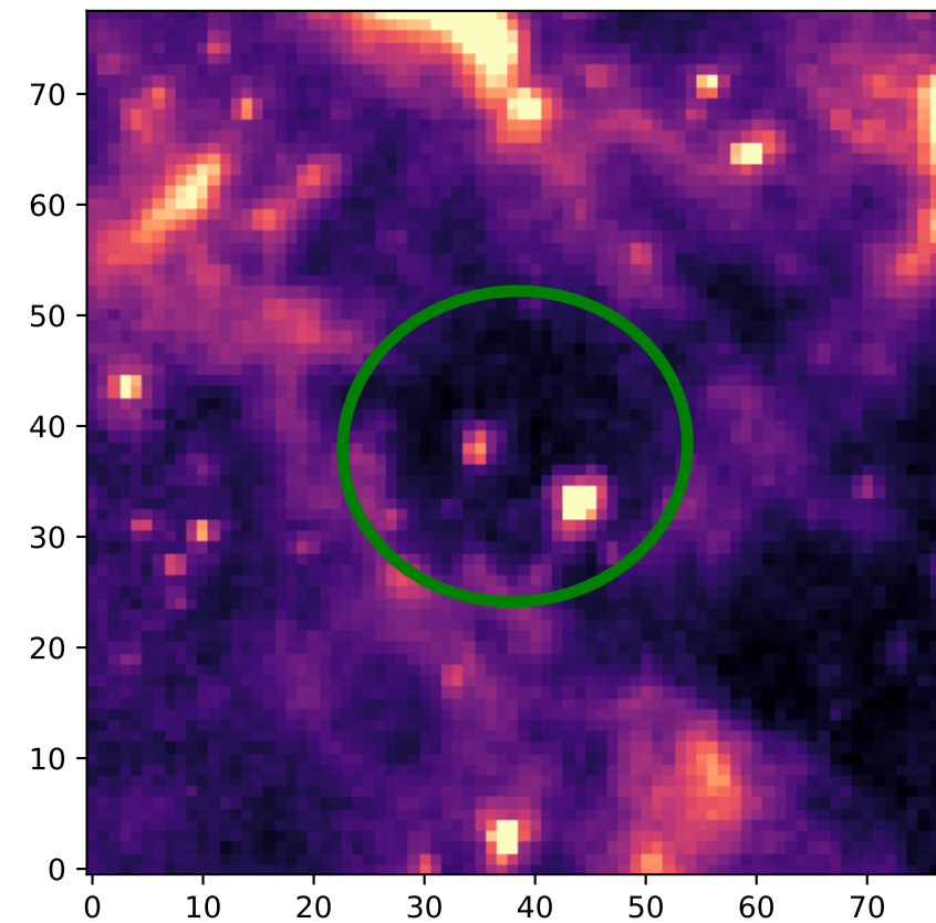
IRAC 8 micron - Classification: Bubble-Like
