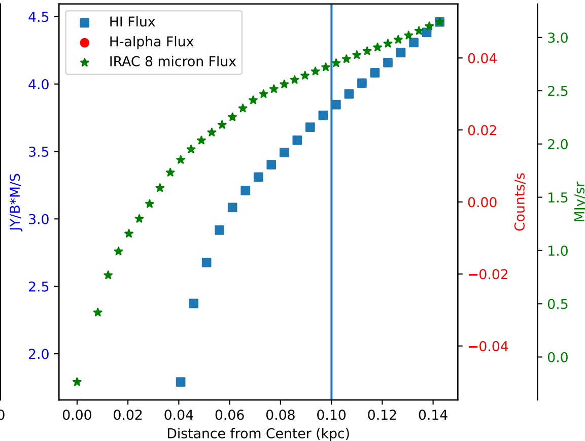
Flux of HI vs. H-alpha in Galaxy: IC10 - Region 5
