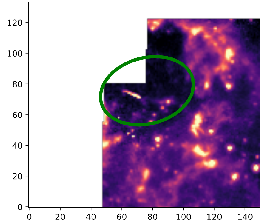
IRAC 8 micron - Classification: Diffuse
