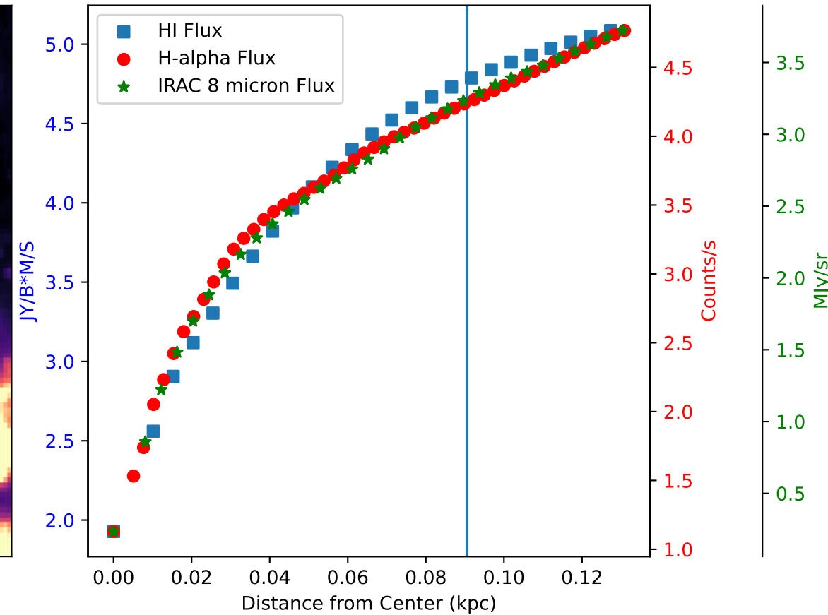
Flux of HI vs. H-alpha in Galaxy: IC10 - Region 6
