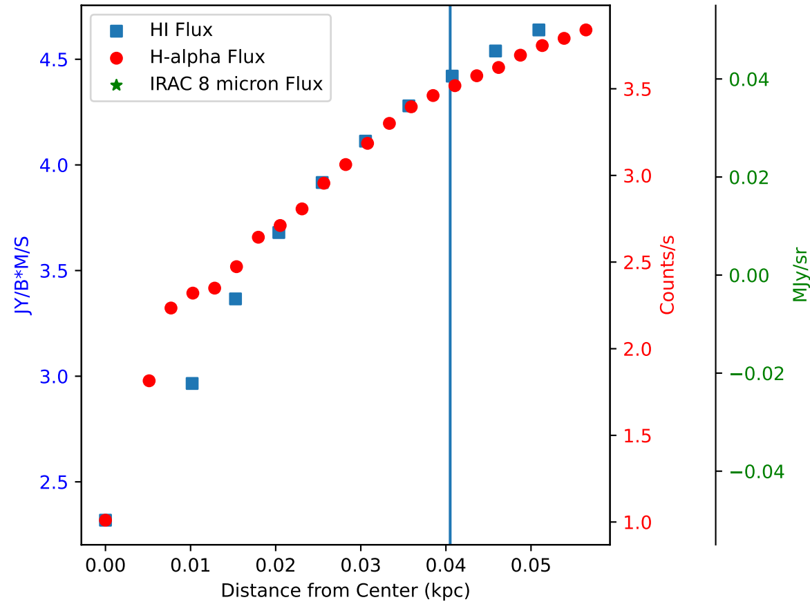
Flux of HI vs. H-alpha in Galaxy: IC10 - Region 1
